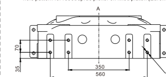
hole pattern for robot/sprue picker on fixed platen (Euromap 18-E8)
