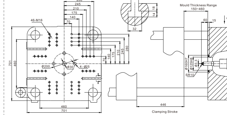
hole pattern for robot/sprue picker on fixed platen (Euromap 18-E8)
