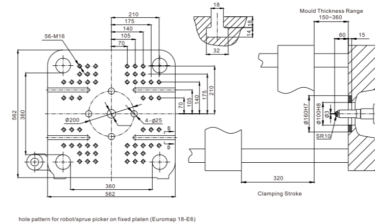
hole pattern for robot/sprue picker on fixed platen (Euromap 18-E6)
