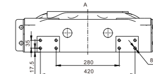
hole pattern for robot/sprue picker on fixed platen (Euromap 18-E6)
